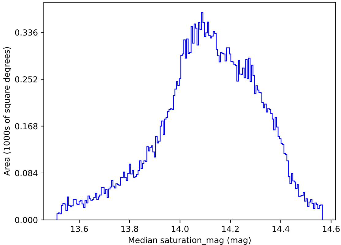
too_elab_r64_d3_griz_v3.4_10yrs All sky all bands: Median saturation_mag
