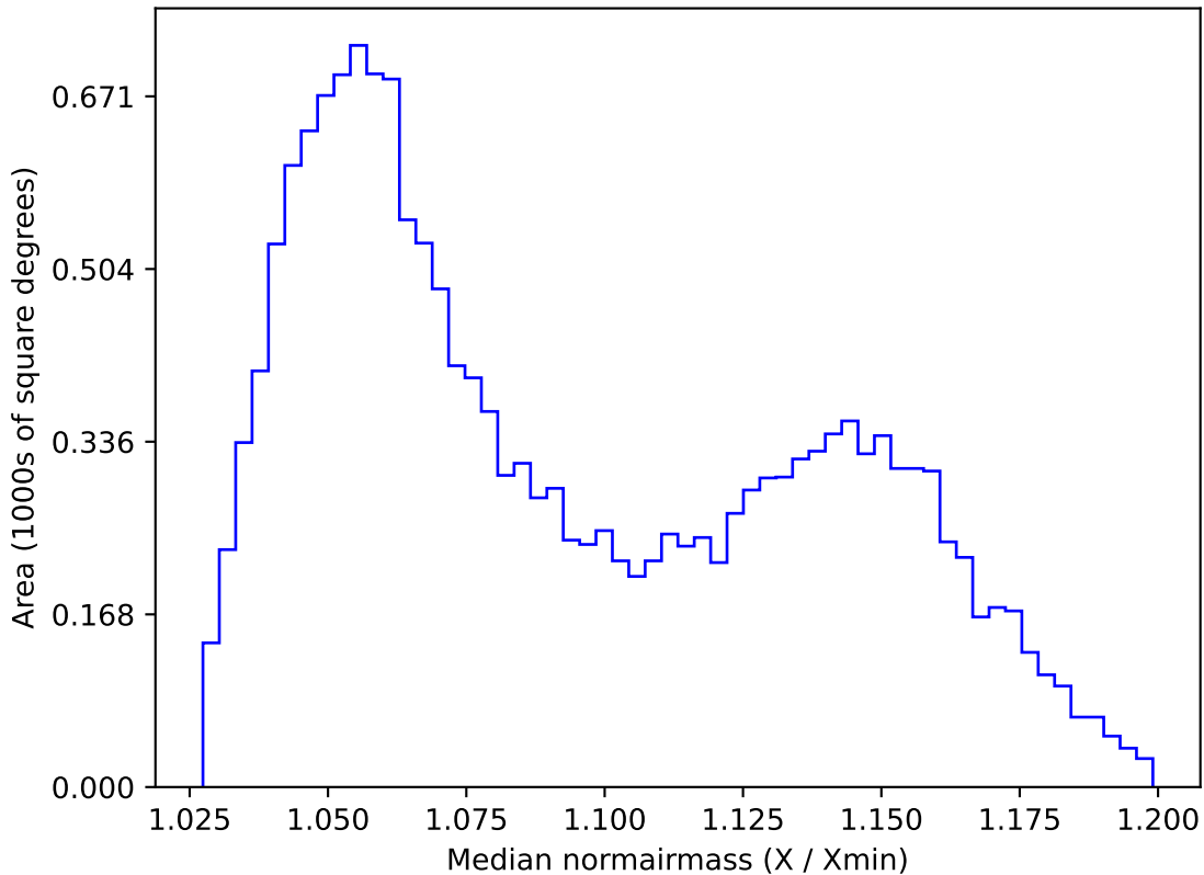
too_elab_r64_d3_griz_v3.4_10yrs WFD y band: Median normairmass
