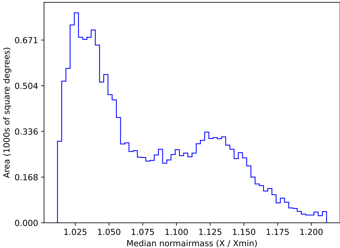
too_elab_r64_d3_griz_v3.4_10yrs WFD u band: Median normairmass
