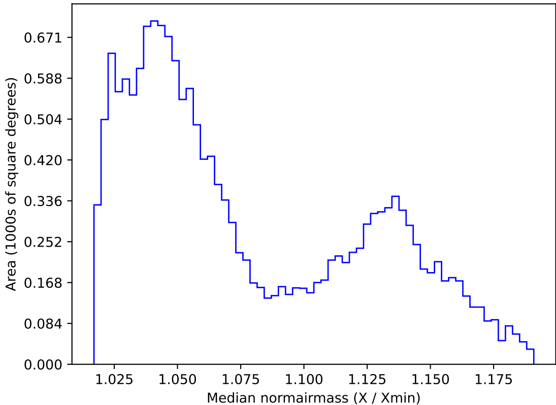
too_elab_r64_d3_griz_v3.4_10yrs WFD r band: Median normairmass
