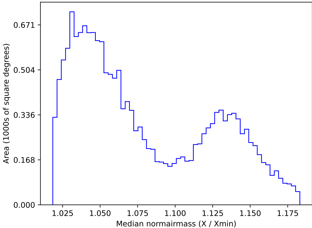
too_elab_r64_d3_griz_v3.4_10yrs WFD i band: Median normairmass
