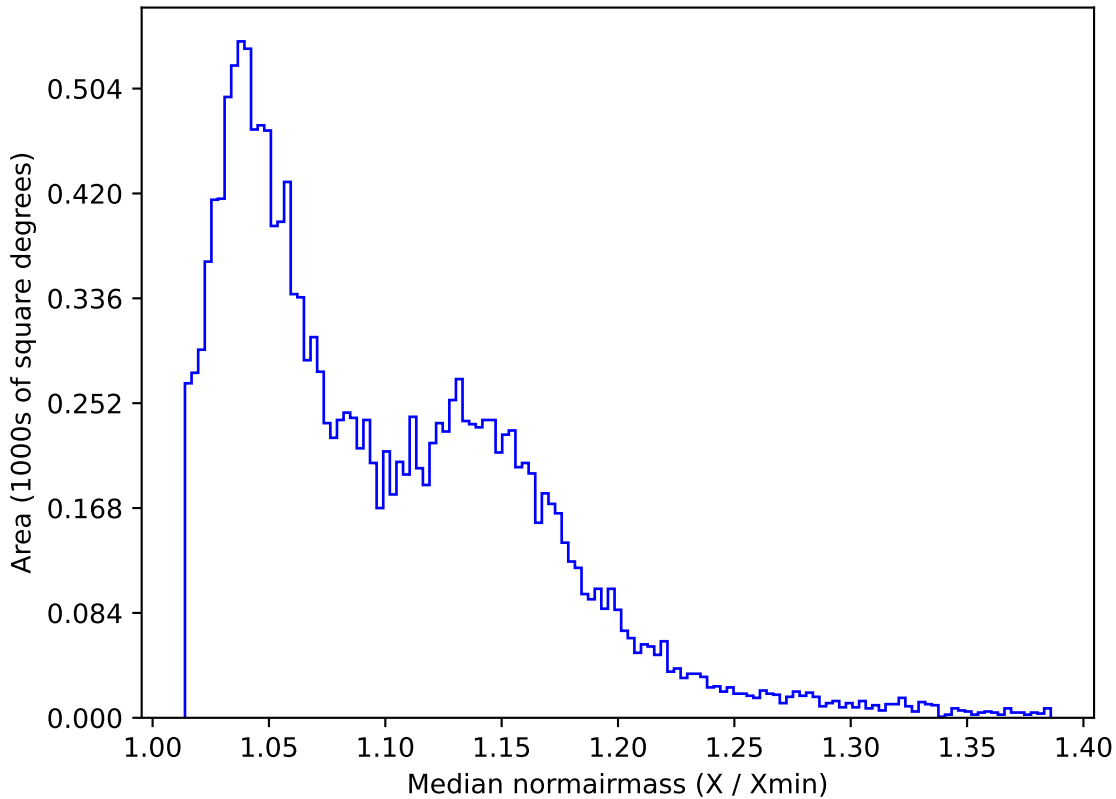
too_elab_r64_d3_griz_v3.4_10yrs WFD g band: Median normairmass
