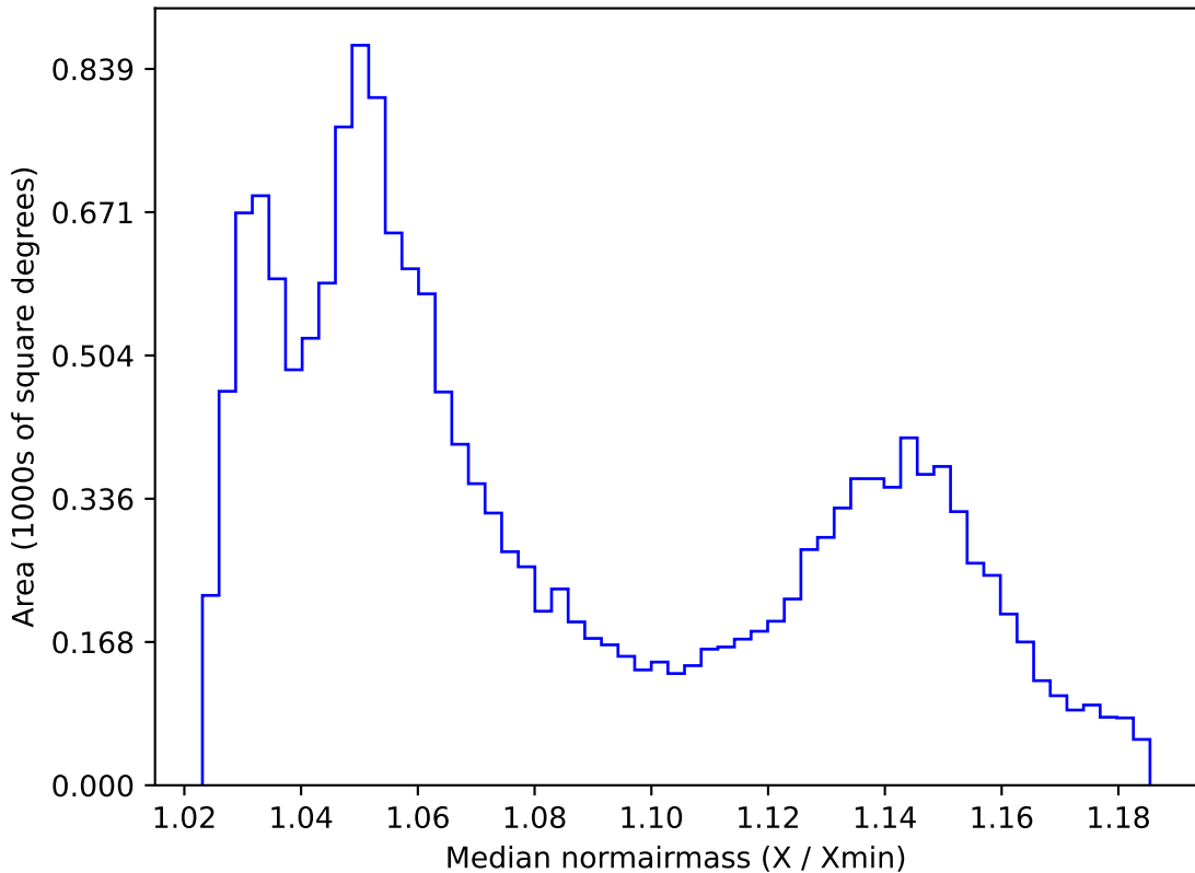
too_elab_r64_d3_griz_v3.4_10yrs WFD all bands: Median normairmass
