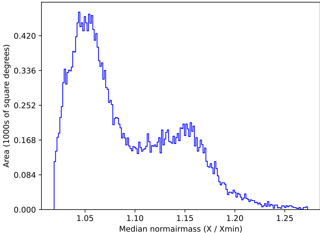
too_elab_r64_d3_griz_v3.4_10yrs All sky z band: Median normairmass
