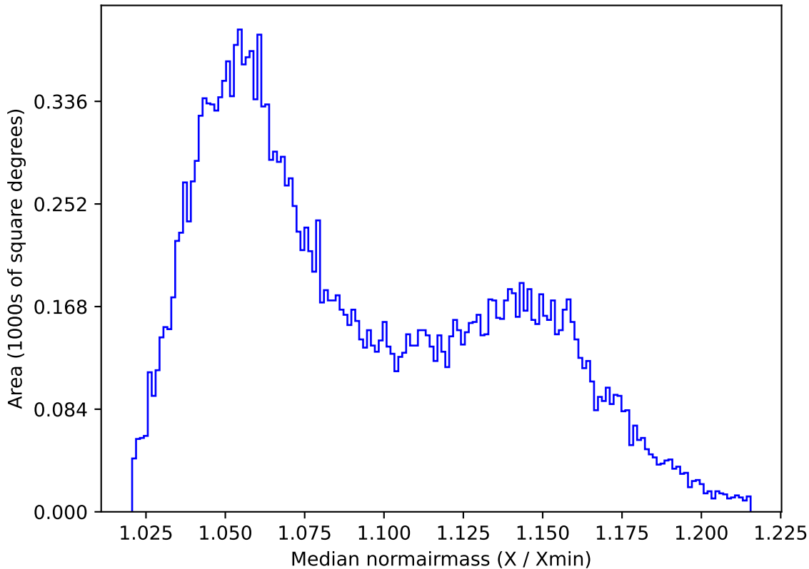
too_elab_r64_d3_griz_v3.4_10yrs All sky y band: Median normairmass
