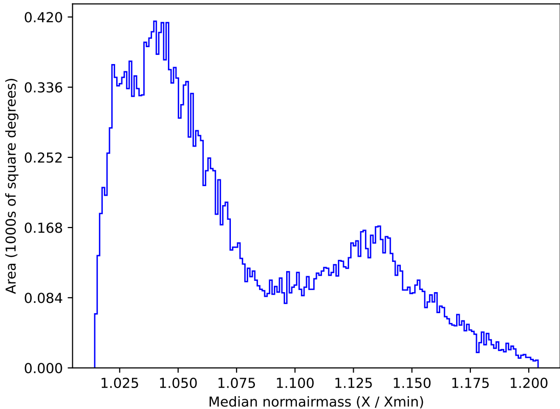
too_elab_r64_d3_griz_v3.4_10yrs All sky r band: Median normairmass
