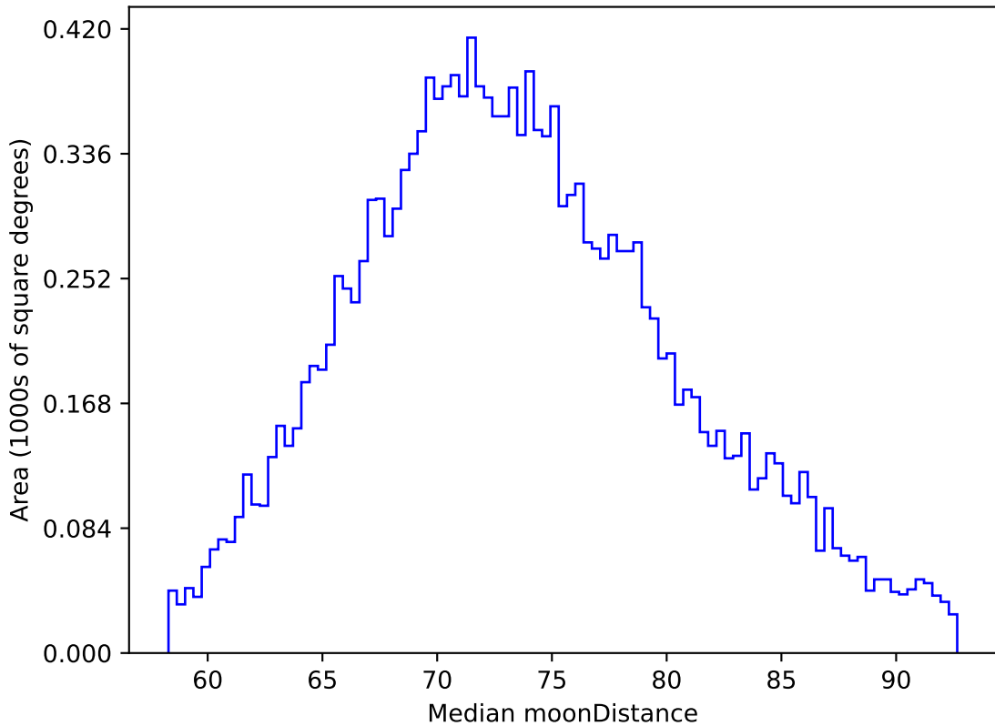
too_elab_r64_d3_griz_v3.4_10yrs WFD z band: Median moonDistance
