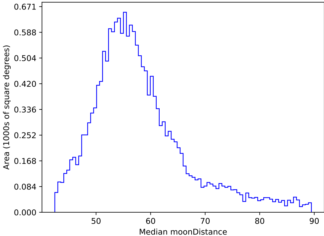
too_elab_r64_d3_griz_v3.4_10yrs WFD y band: Median moonDistance
