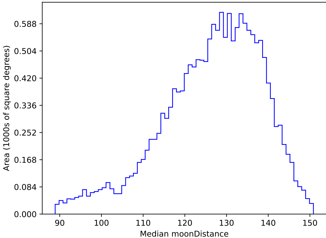
too_elab_r64_d3_griz_v3.4_10yrs WFD u band: Median moonDistance
