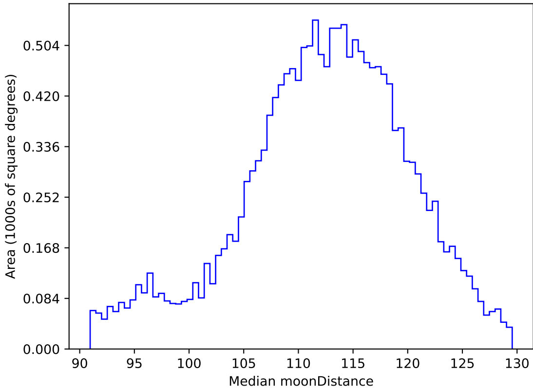
too_elab_r64_d3_griz_v3.4_10yrs WFD r band: Median moonDistance
