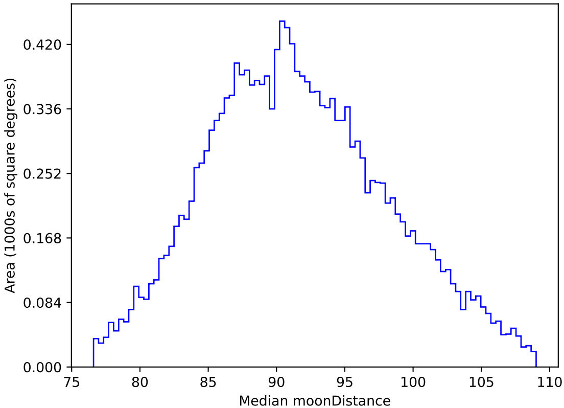
too_elab_r64_d3_griz_v3.4_10yrs WFD i band: Median moonDistance
