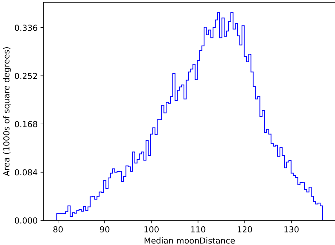
too_elab_r64_d3_griz_v3.4_10yrs WFD g band: Median moonDistance
