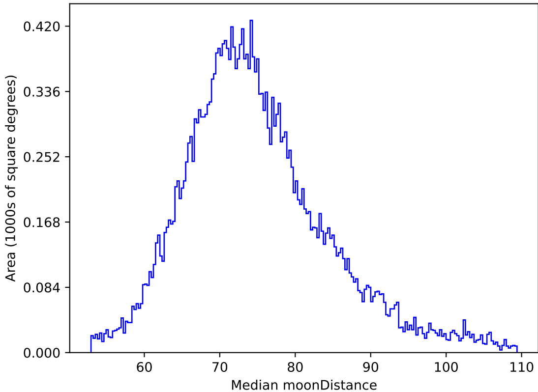
too_elab_r64_d3_griz_v3.4_10yrs All sky z band: Median moonDistance
