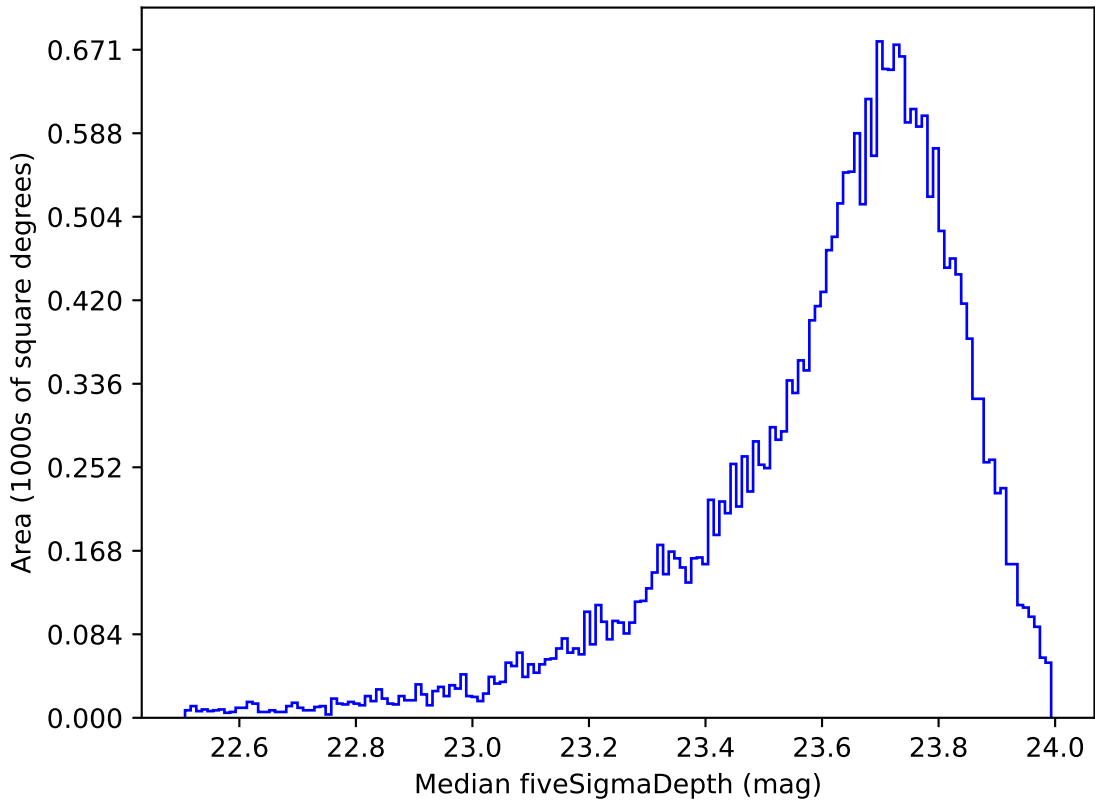
too_elab_r64_d3_griz_v3.4_10yrs Yr 1 i band: Median fiveSigmaDepth
