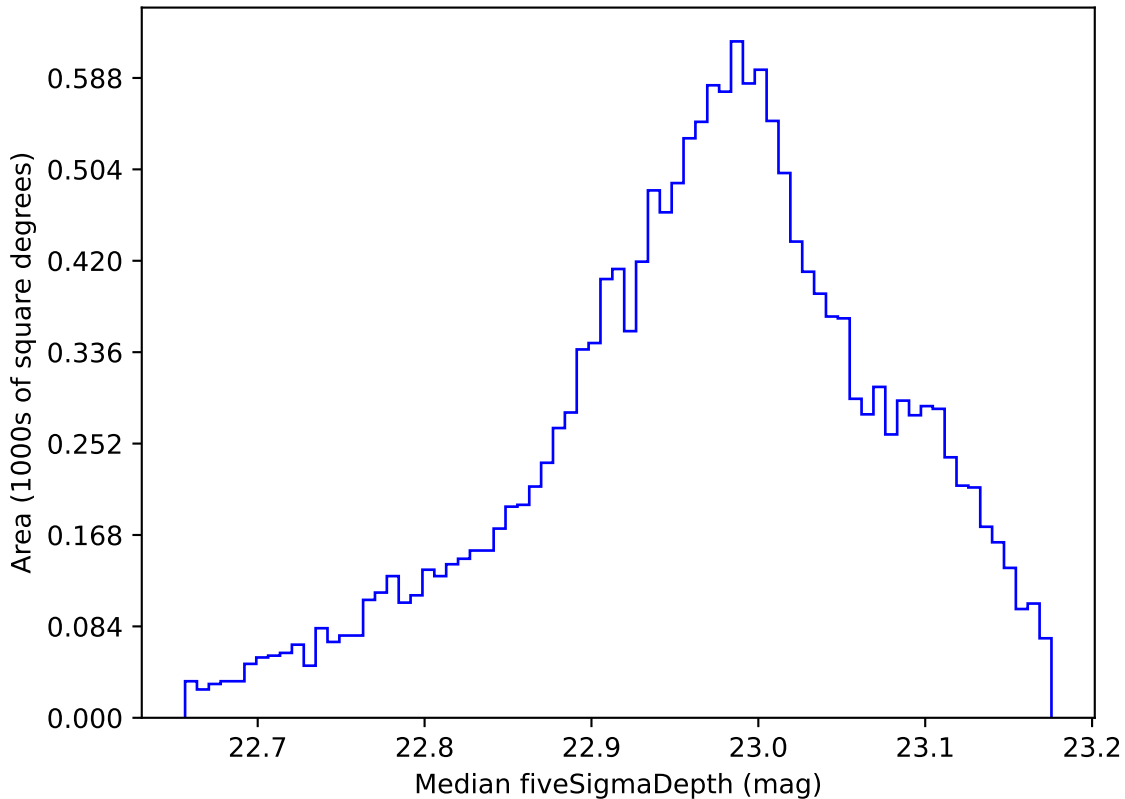
too_elab_r64_d3_griz_v3.4_10yrs WFD z band: Median fiveSigmaDepth
