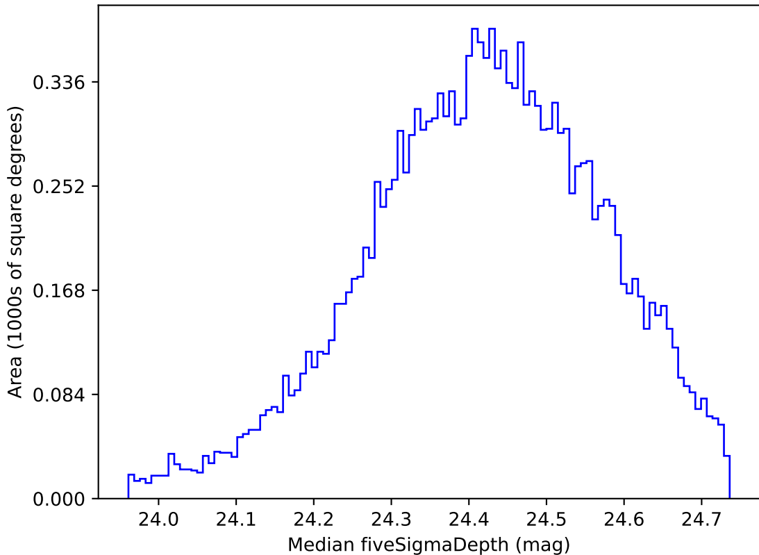
too_elab_r64_d3_griz_v3.4_10yrs WFD g band: Median fiveSigmaDepth
