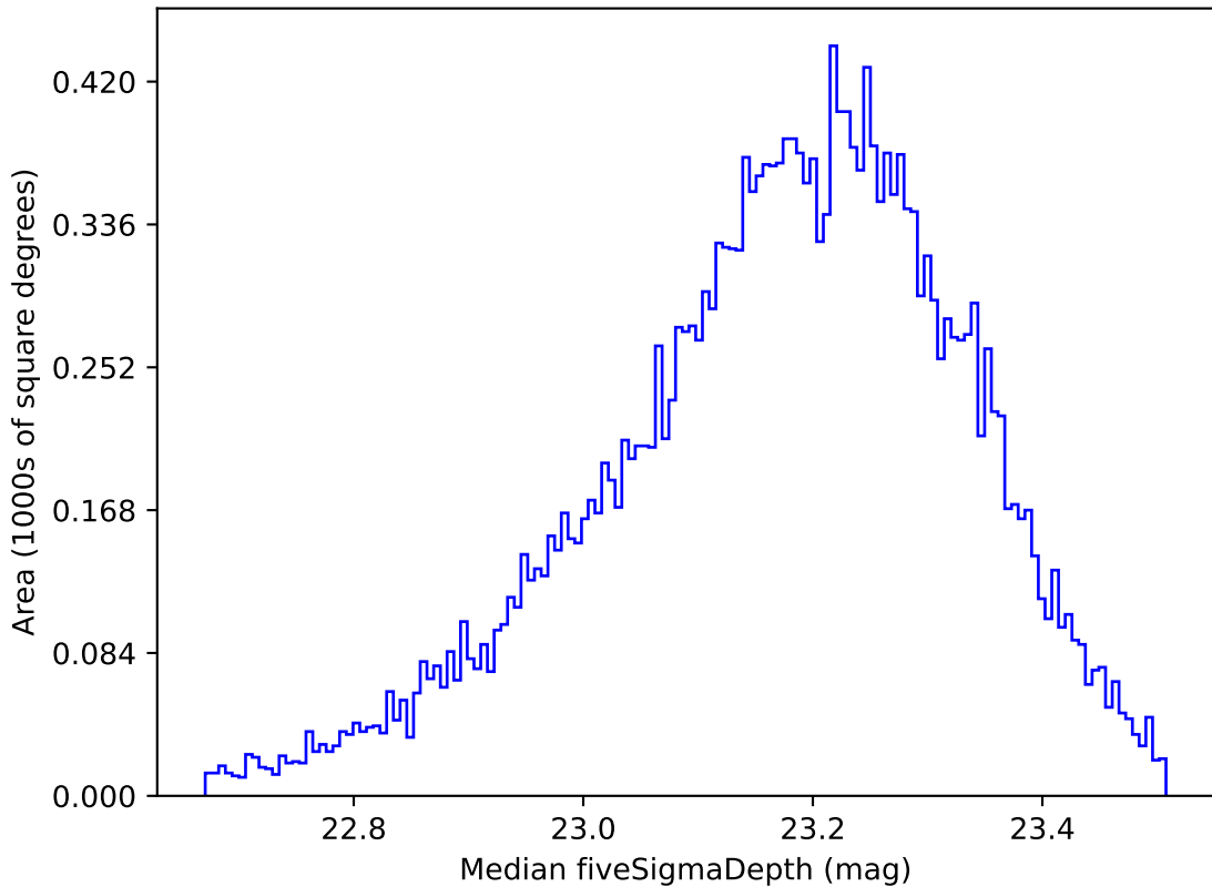
too_elab_r64_d3_griz_v3.4_10yrs All sky u band: Median fiveSigmaDepth
