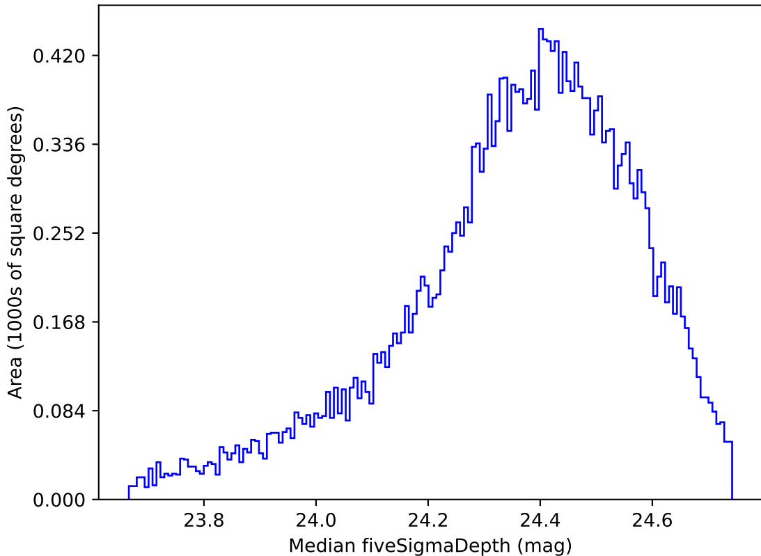
too_elab_r64_d3_griz_v3.4_10yrs All sky g band: Median fiveSigmaDepth
