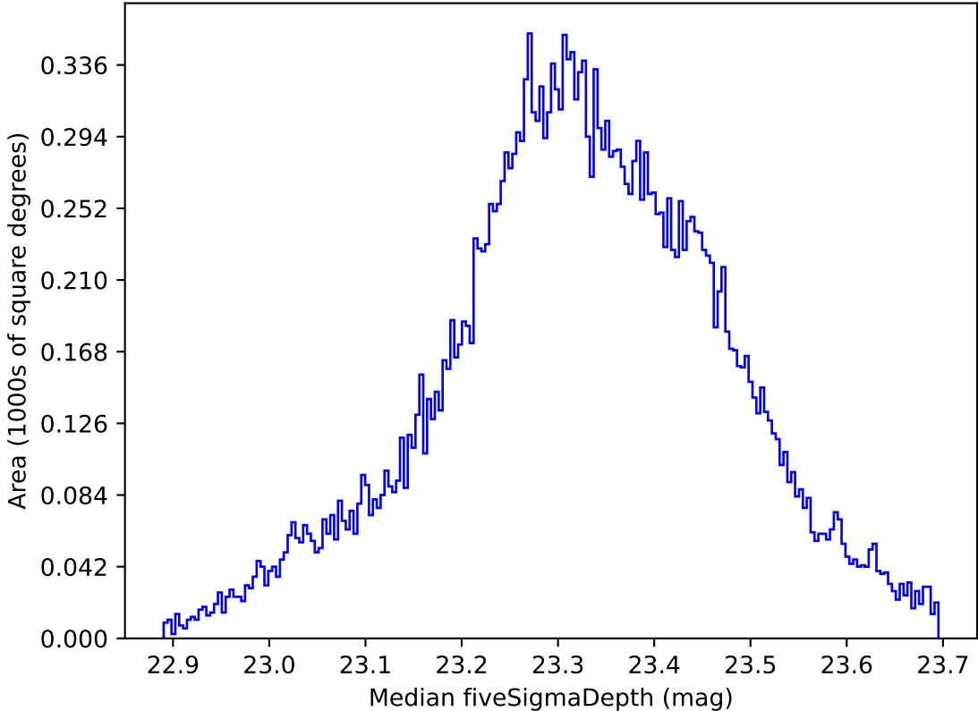
too_elab_r64_d3_griz_v3.4_10yrs All sky all bands: Median fiveSigmaDepth
