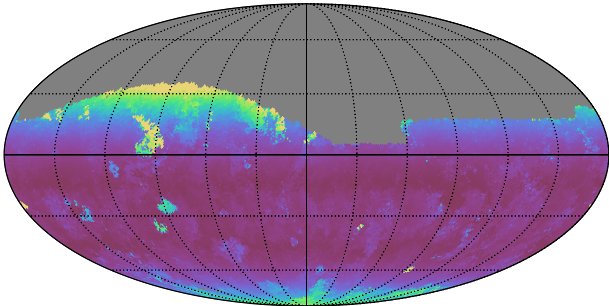
too_elab_r64_d3_griz_v3.4_10yrs Yr 1 z band: Median airmass
