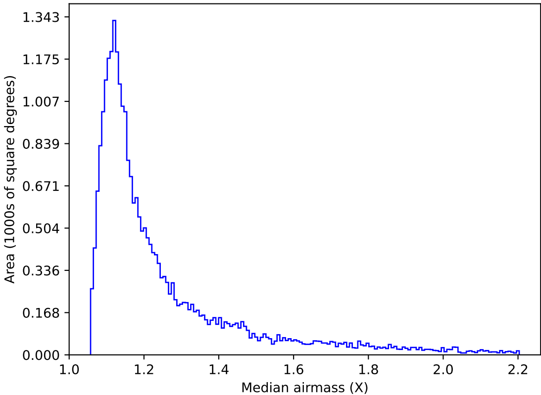
too_elab_r64_d3_griz_v3.4_10yrs Yr 1 z band: Median airmass
