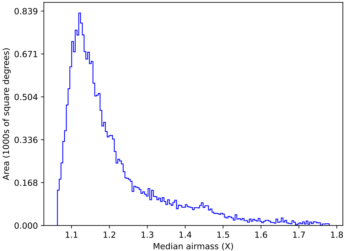
too_elab_r64_d3_griz_v3.4_10yrs Yr 1 y band: Median airmass
