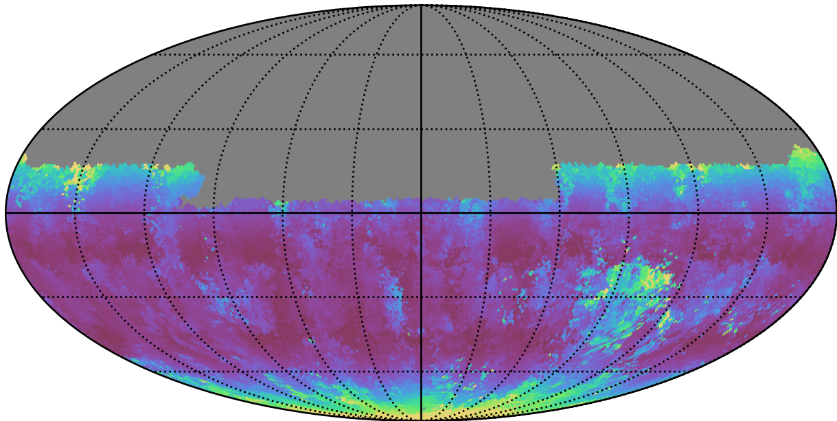
too_elab_r64_d3_griz_v3.4_10yrs Yr 1 u band: Median airmass
