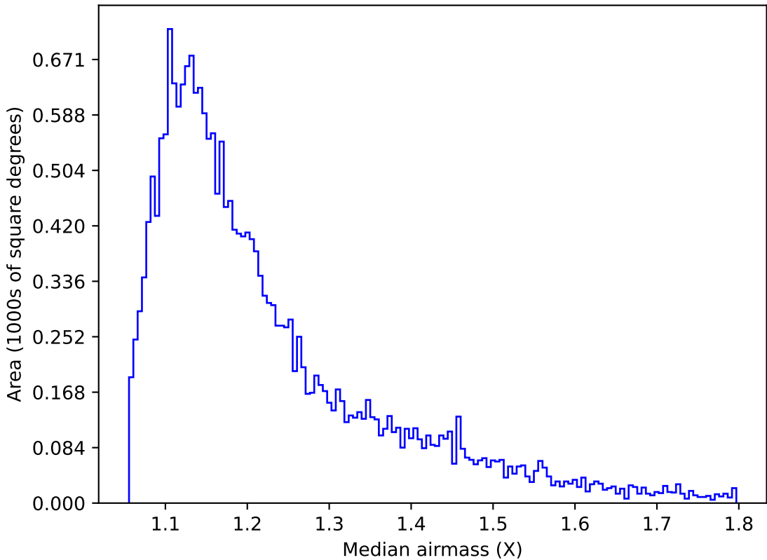
too_elab_r64_d3_griz_v3.4_10yrs Yr 1 u band: Median airmass
