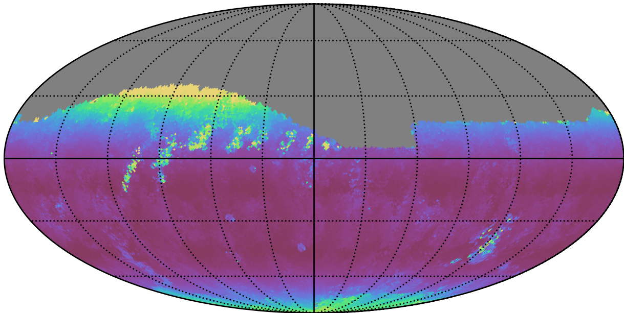
too_elab_r64_d3_griz_v3.4_10yrs Yr 1 r band: Median airmass
