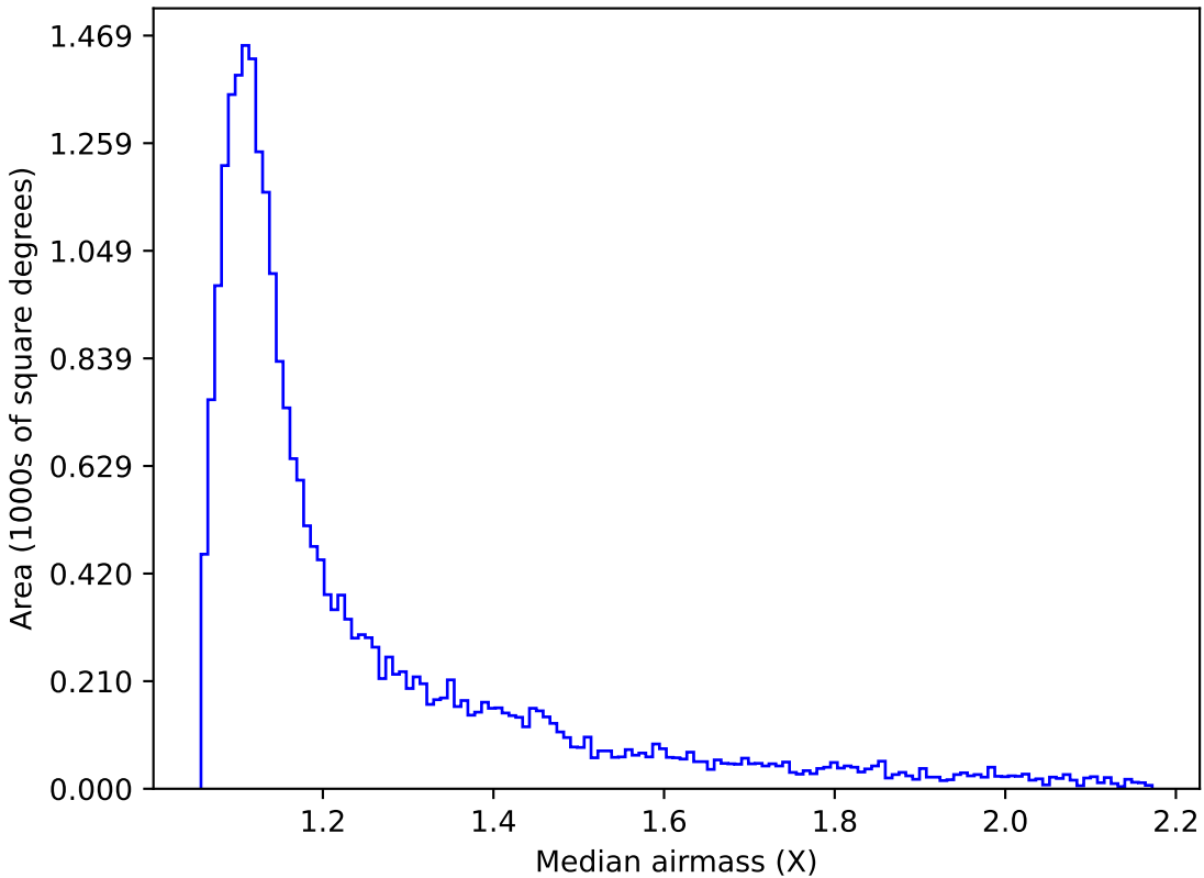
too_elab_r64_d3_griz_v3.4_10yrs Yr 1 r band: Median airmass
