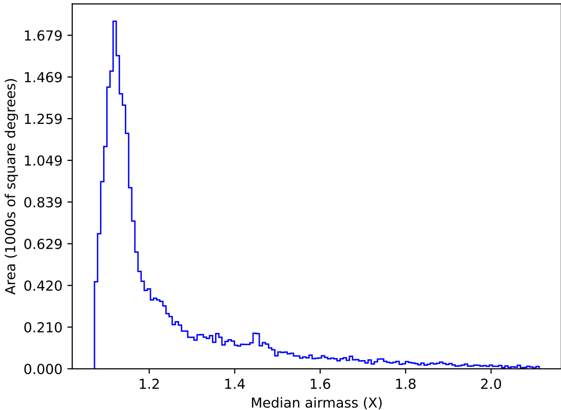
too_elab_r64_d3_griz_v3.4_10yrs Yr 1 all bands: Median airmass
