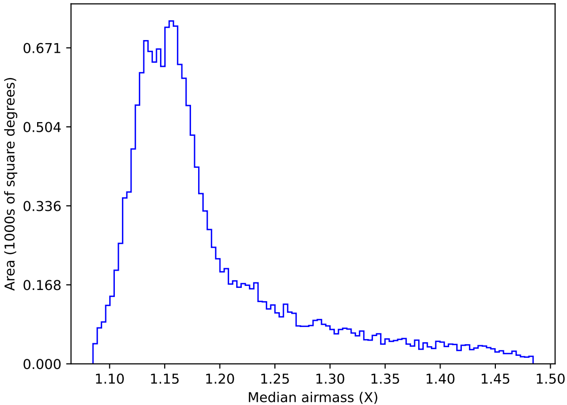
too_elab_r64_d3_griz_v3.4_10yrs WFD z band: Median airmass
