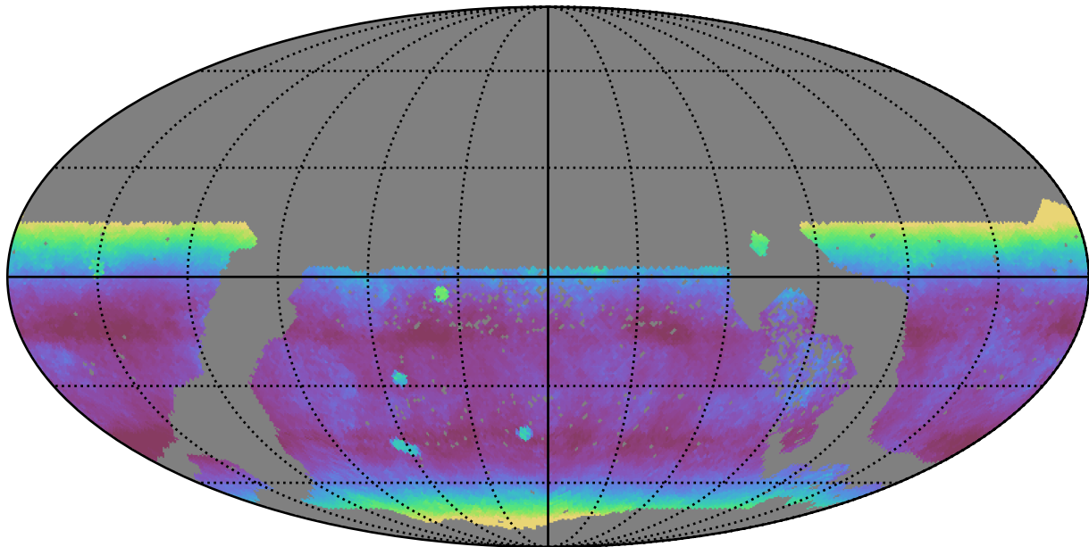
too_elab_r64_d3_griz_v3.4_10yrs WFD y band: Median airmass
