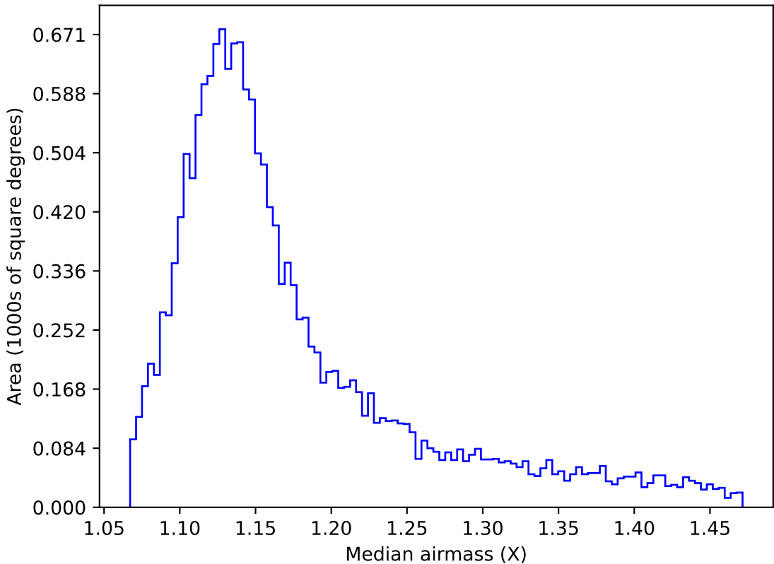
too_elab_r64_d3_griz_v3.4_10yrs WFD u band: Median airmass
