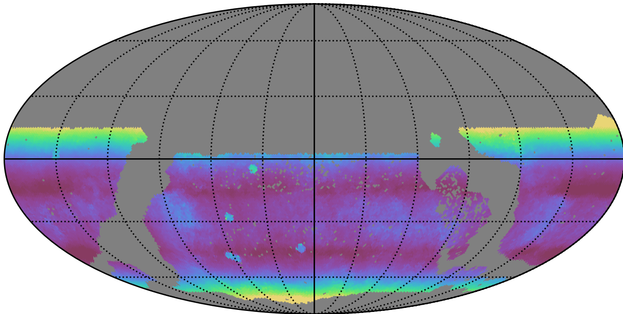
too_elab_r64_d3_griz_v3.4_10yrs WFD r band: Median airmass
