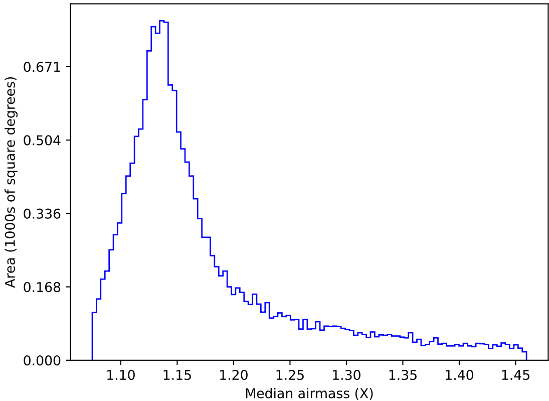
too_elab_r64_d3_griz_v3.4_10yrs WFD r band: Median airmass
