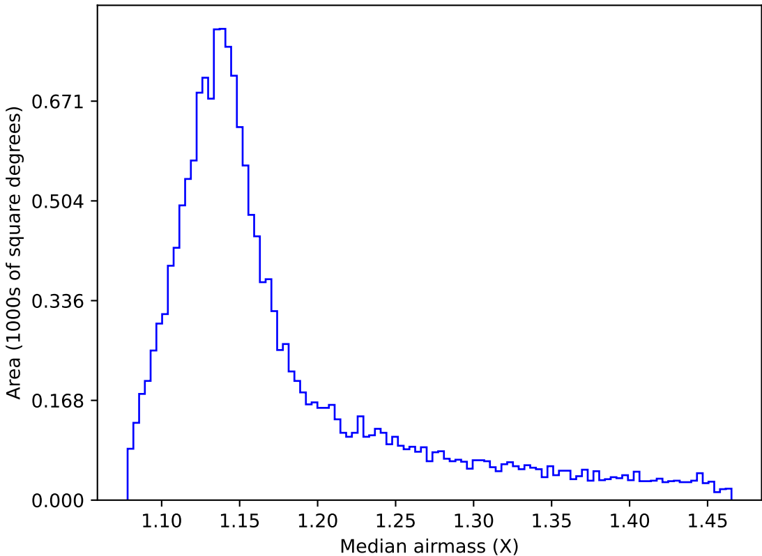
too_elab_r64_d3_griz_v3.4_10yrs WFD i band: Median airmass
