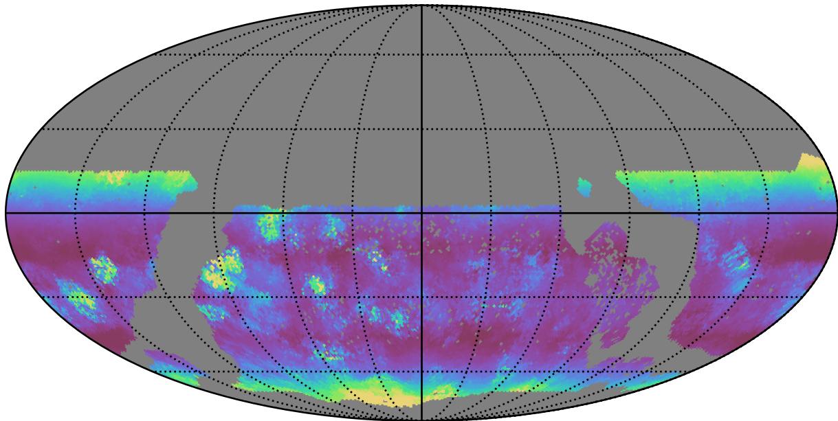
too_elab_r64_d3_griz_v3.4_10yrs WFD g band: Median airmass
