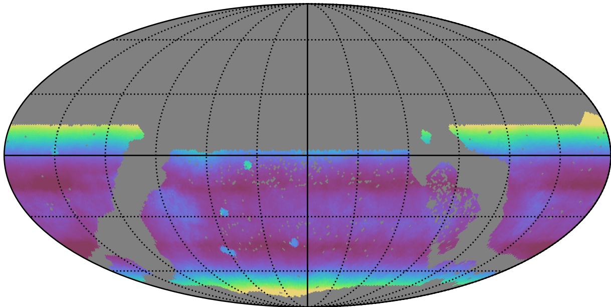
too_elab_r64_d3_griz_v3.4_10yrs WFD all bands: Median airmass
