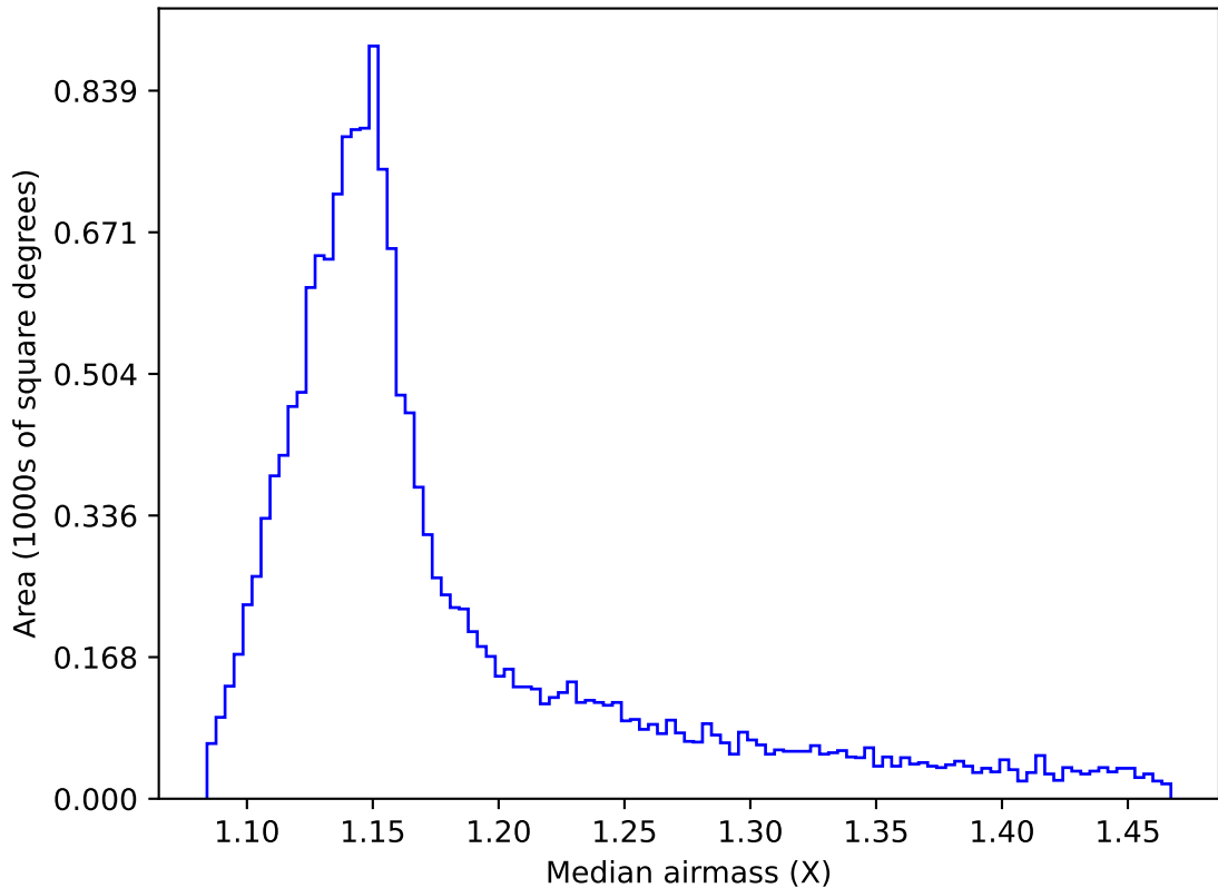
too_elab_r64_d3_griz_v3.4_10yrs WFD all bands: Median airmass
