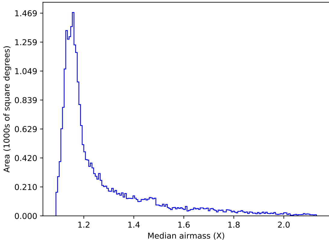
too_elab_r64_d3_griz_v3.4_10yrs All sky z band: Median airmass
