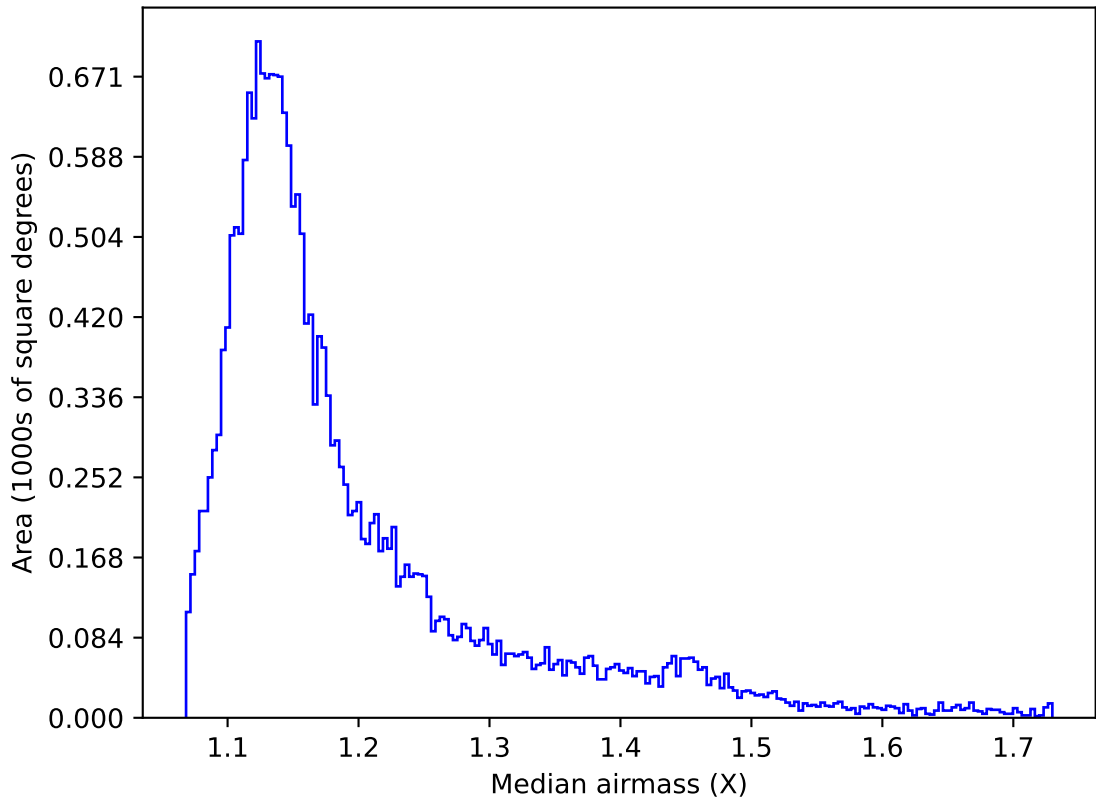
too_elab_r64_d3_griz_v3.4_10yrs All sky u band: Median airmass
