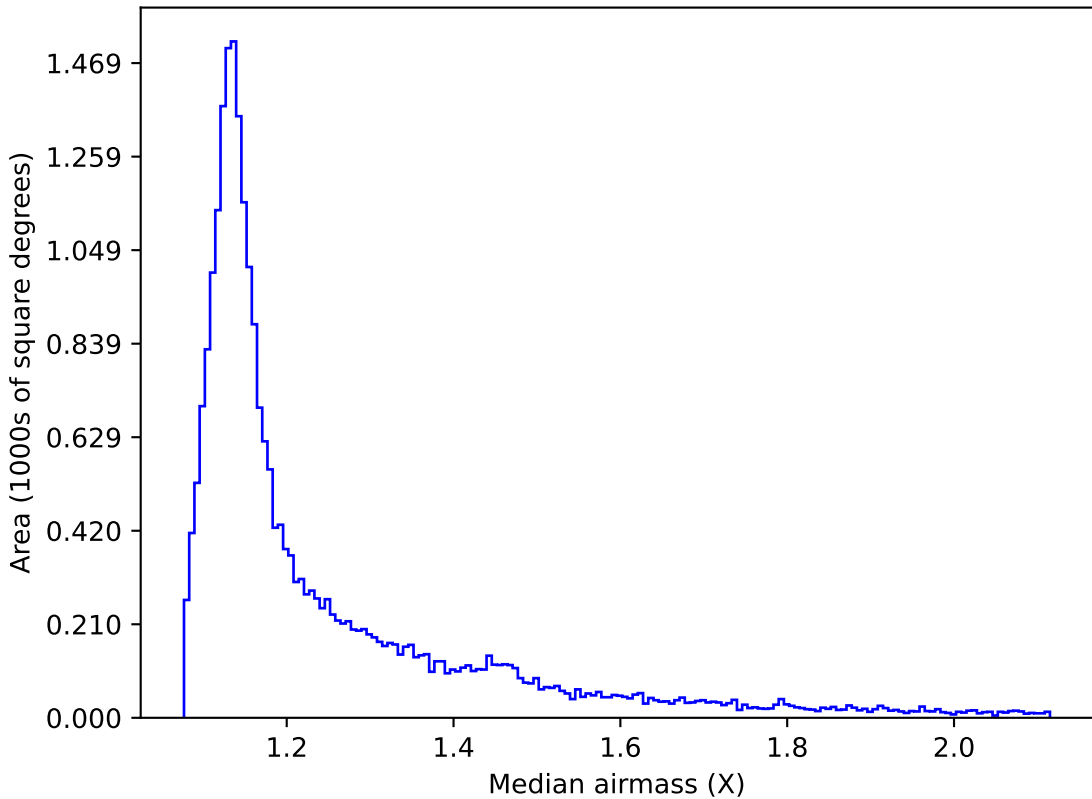
too_elab_r64_d3_griz_v3.4_10yrs All sky r band: Median airmass
