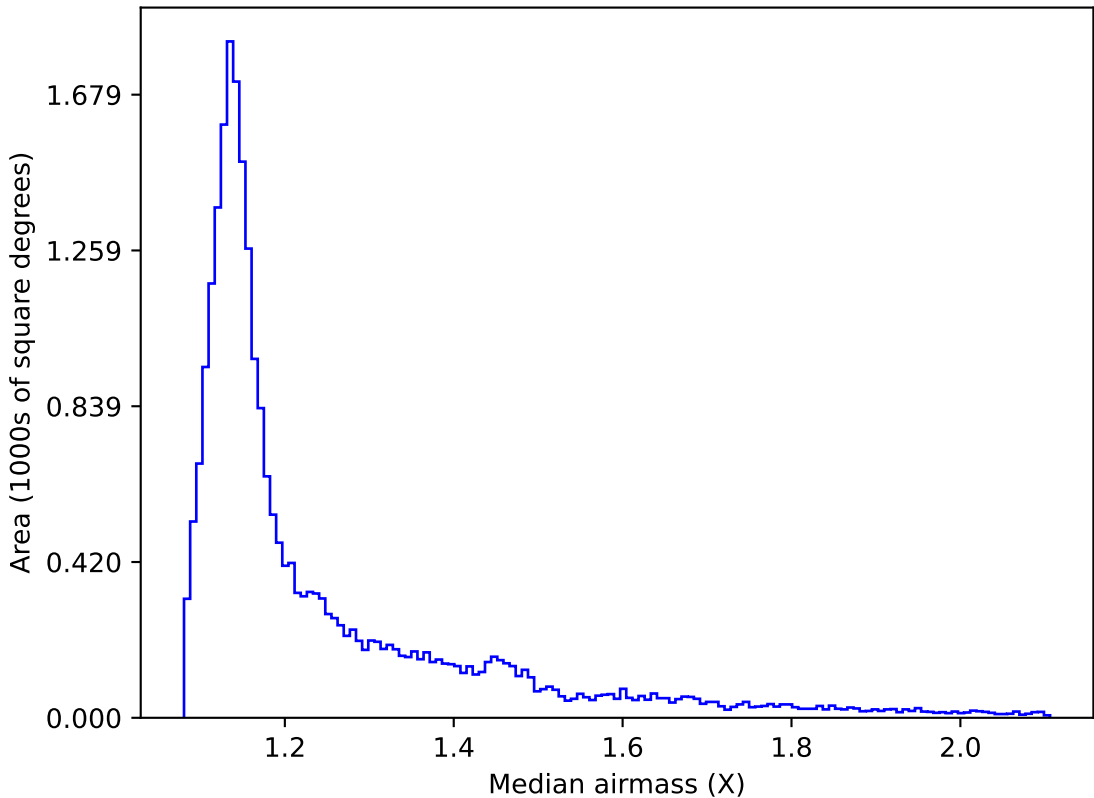
too_elab_r64_d3_griz_v3.4_10yrs All sky i band: Median airmass
