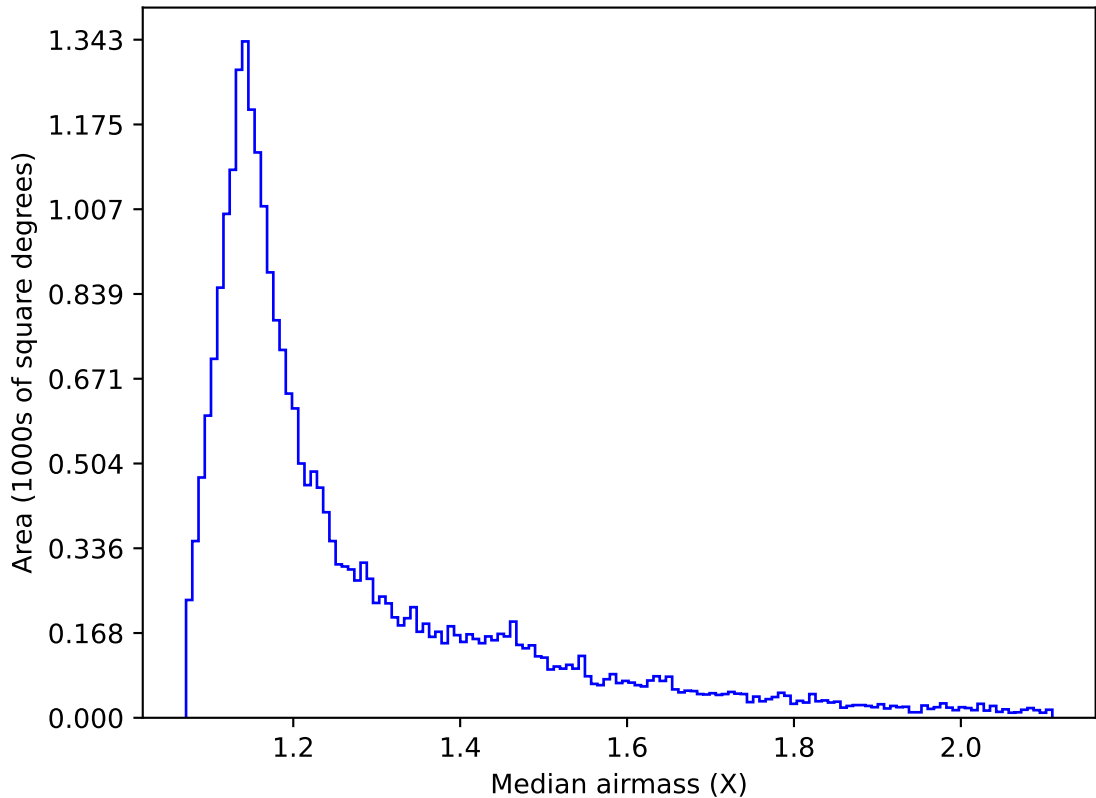
too_elab_r64_d3_griz_v3.4_10yrs All sky g band: Median airmass
