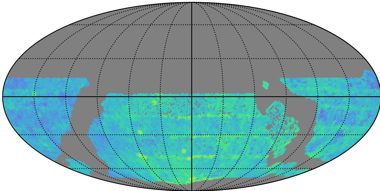
too_elab_r64_d3_griz_v3.4_10yrs WFD z band: Median Season Length
