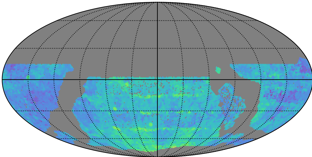
too_elab_r64_d3_griz_v3.4_10yrs WFD y band: Median Season Length
