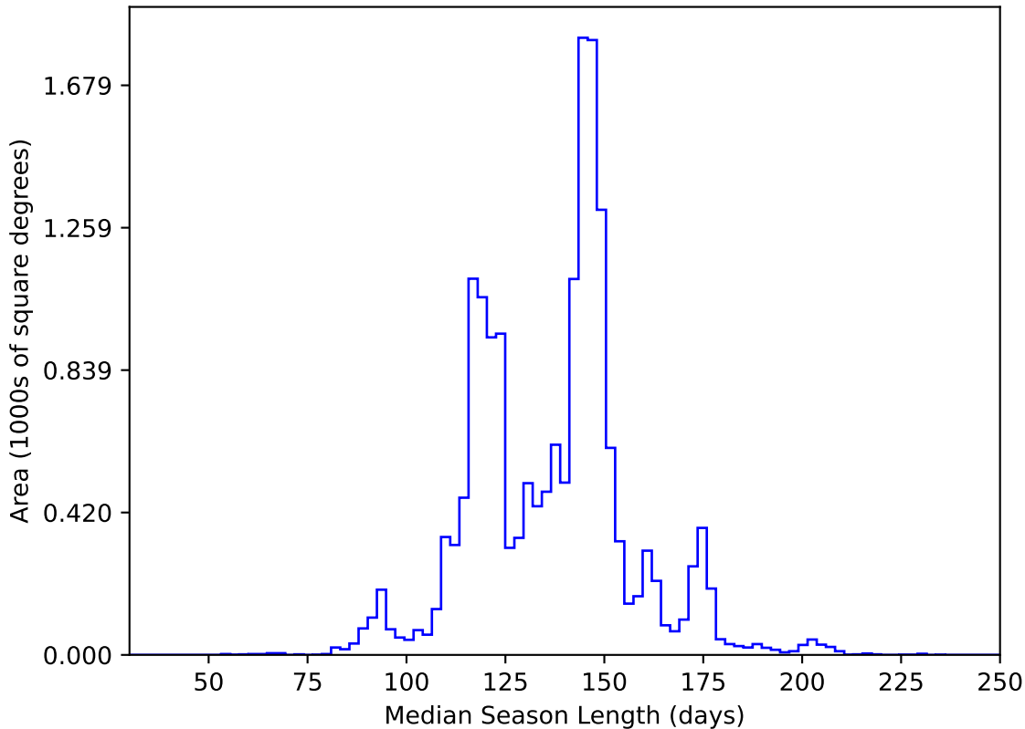
too_elab_r64_d3_griz_v3.4_10yrs WFD y band: Median Season Length
