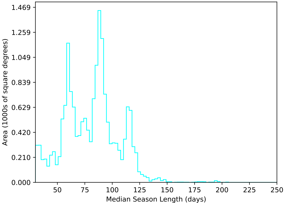
too_elab_r64_d3_griz_v3.4_10yrs WFD u band: Median Season Length
