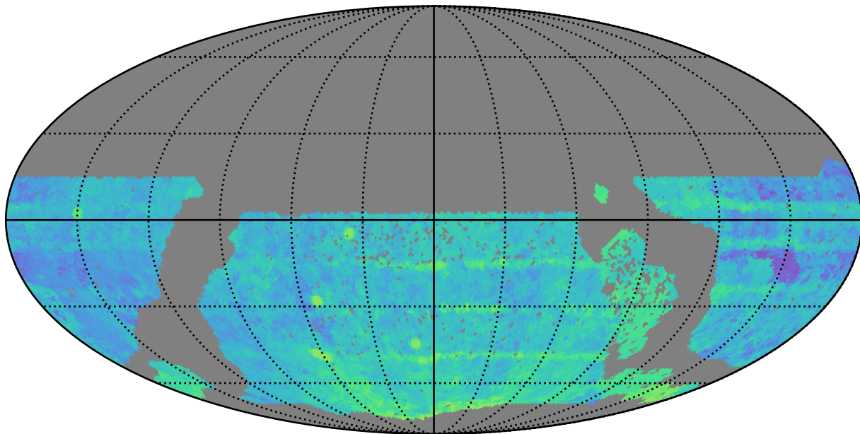
too_elab_r64_d3_griz_v3.4_10yrs WFD r band: Median Season Length
